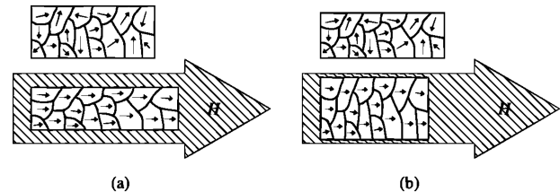
Figure 1: Positive (a) and negative (b) magnetostriction
