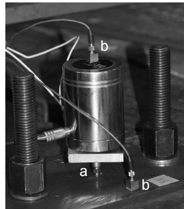
Figure 7 – Test : load cell (a) and unidirectional accelerometers (b)
