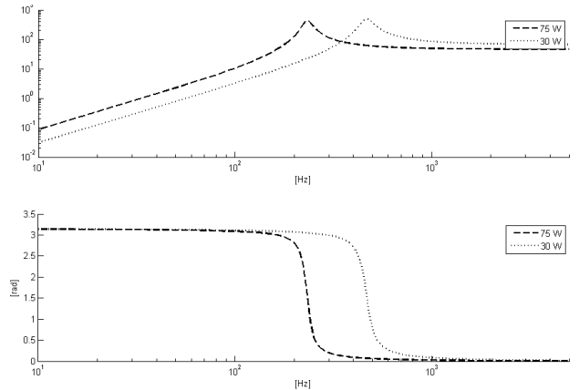
Figure 5 – Theoretical transfer functions of M.A. tested (magnitude and phase)
