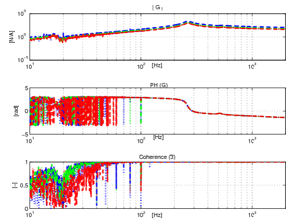
Figure 10 – E.75W MA. Experimental transfer function G_3(s)=F_T/I obtained with harmonic excitation for different value of current.
