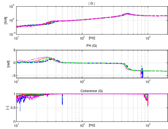
Figure 9 - E.30W MA. Experimental transfer function G_3(s)=F_T/I obtained with sweep-sine excitation for different value of current.
