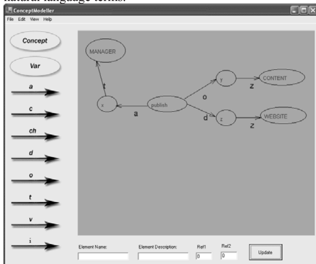
Figure 2. 'Publish' event frame visualization in ConceptModeller and the frame fragment XML representation in the database
