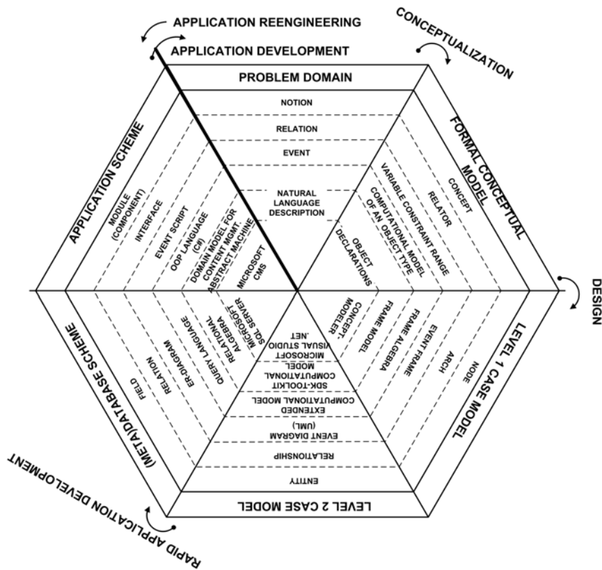
Figure 1. Complex software application development diagram
