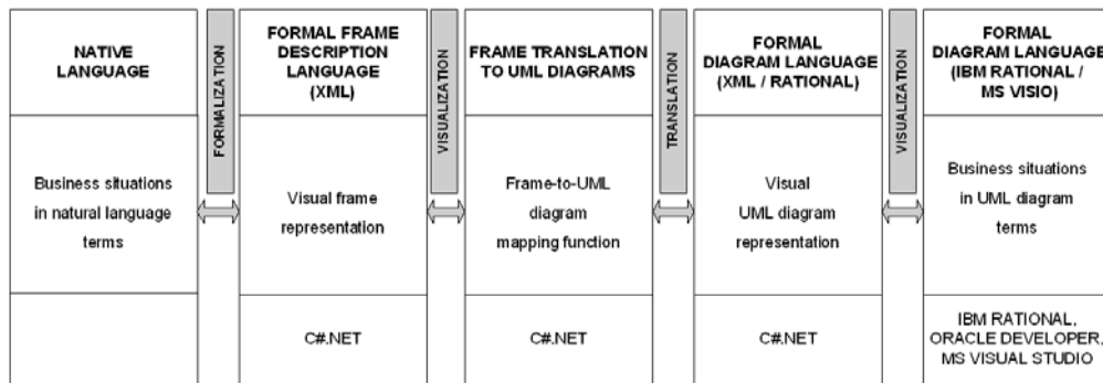
Figure 3. ConceptModeller translation scheme
