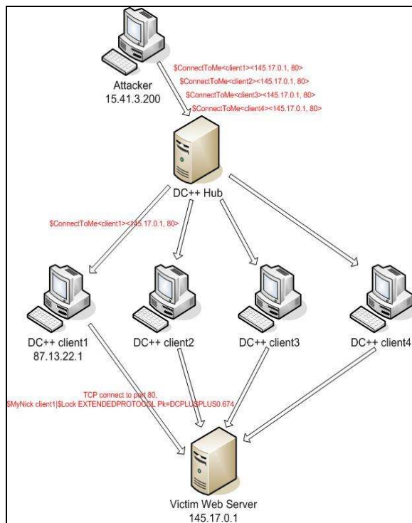
Figure 2: A DC++ DDoS attack in action
