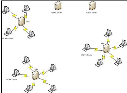
Figure 1. DC++ network architecture
