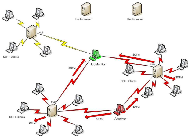
Figure 3: Detecting the attacker hubs
