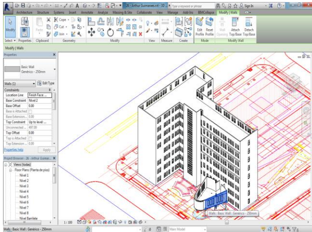
Figure 3 - BIM model of the old School of Engineering of the UFMG
